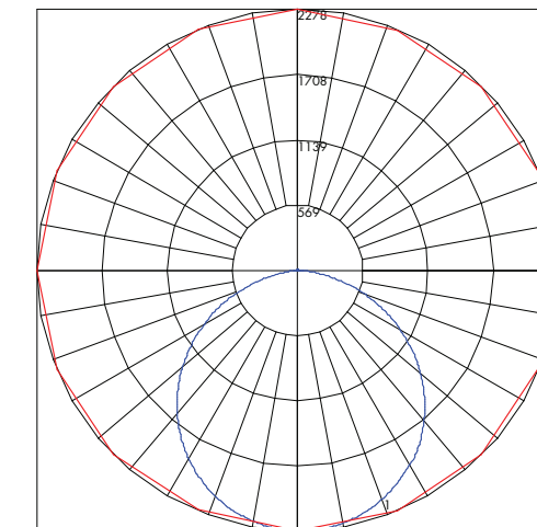
Maximum Candela = 2277.7 Located At Horizontal Angle = 90, Vertical Angle = -5 # 1 - Vertical Plane Through Horizontal Angles [90 - 270] (Through Max. Cd.) # 2 - Horizontal Cone Through Vertical Angle (.5) (Through Max. Cd.)
